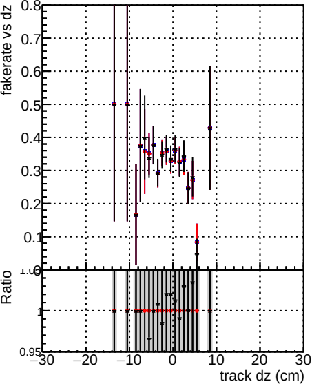
Fake rate vs dz Legend: DOM original original vector 1000evt original 1000evt DOM fitted 1000evt
