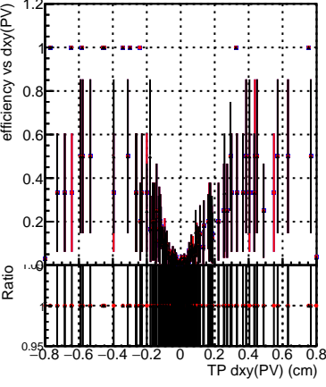
Legend: DQM_original_originalvector_1000evt (blue square), DQM_original_1000evt (red square), DQM_fitted4_1000evt (black square)
