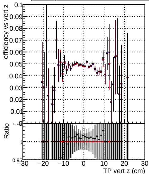
Efficiency vs. TP vert z (cm) Legend: - DQM_original_originalvector_1000evt (blue line with circles) - DQM_original_1000evt (red line with circles) - DQM_fitted4_1000evt (black line with circles)
