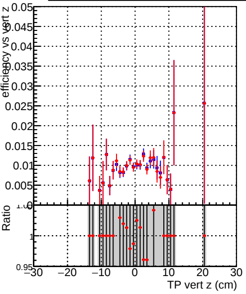
Efficiency vs TP vert z (cm) Legend: DQM_original_1000evt (blue squares), DQM_fitted4_1000evt (red circles)
