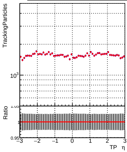
N of simulated tracks vs \eta Legend: DQM_original_1000evt (blue line with dots), DQM_fitted4_1000evt (red line with dots)
