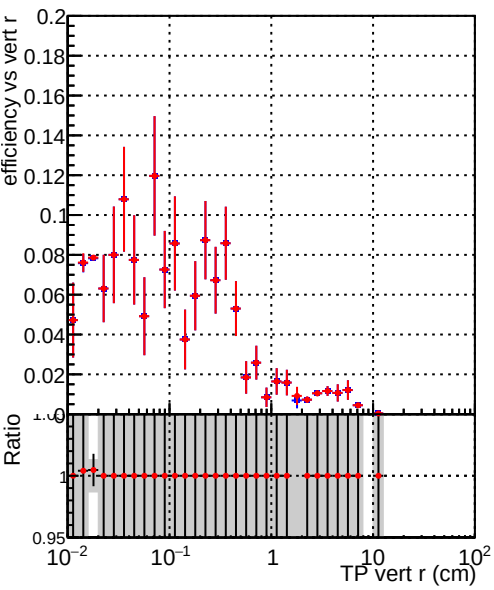
Efficiency vs vertpos Legend: DQM_original_1000evt (blue line with squares), DQM_fitted4_1000evt (red line with circles)
