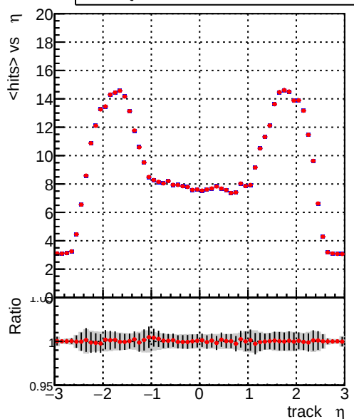
mean hits vs \eta Legend: DQM_original_1000evt (blue line), DQM_fitted4_1000evt (red line)
