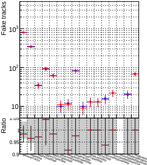
Number —●— DQM_fitted4_1000ev
