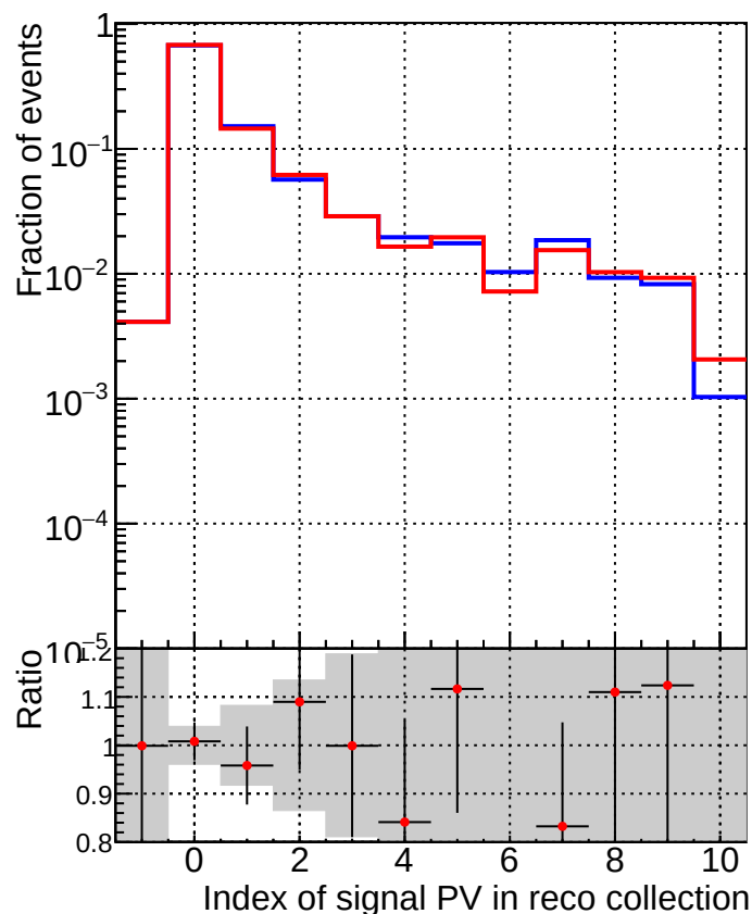
TruePVLocationIndexInRecoVertexCollection
