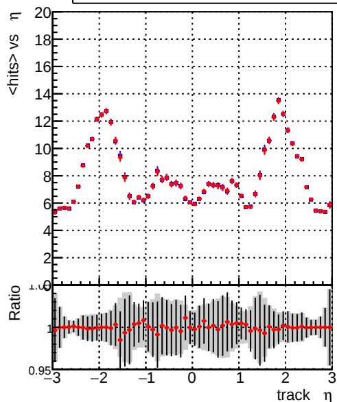
mean hits vs \eta Legend: DQM_original_1000evt (blue line), DQM_fitted4_1000evt (red line)
