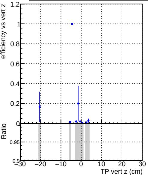
Efficiency vs vert z DQM_V0001_R0000000001_Global_CMSSW_X_Y_Z_RECO
