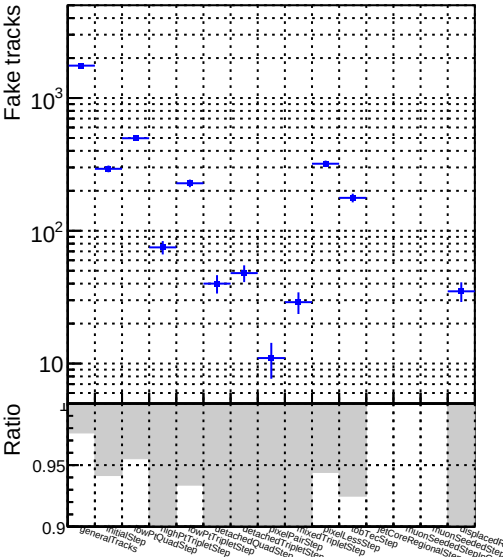
Number DQM_V0001_R000000001_Global_CMSSW_X_Y_Z_RECO
