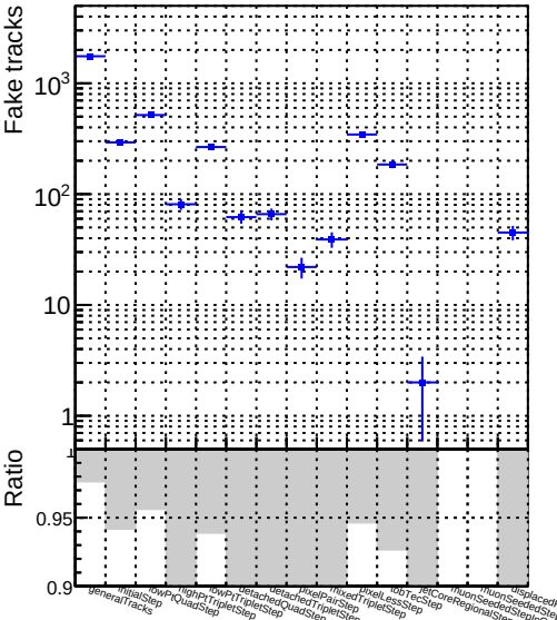
Number DQM_V0001_R000000001_Global_CMSSW_X_Y_Z_RECO
