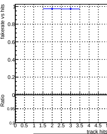
DQM_V0001_R000000001_Global_CMSSW_X_Y_Z_RECO
