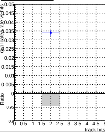
Duplicates Rate vs
