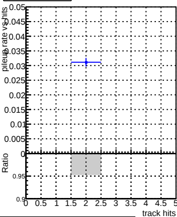
Pileup rate vs
