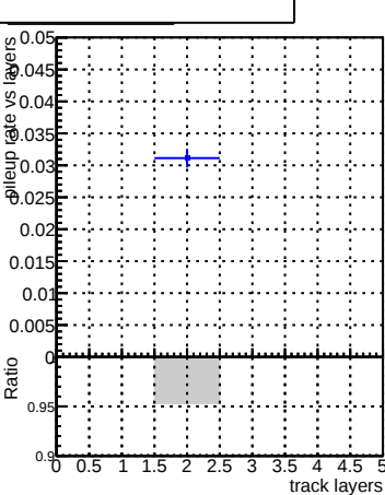
Pileup rate vs
