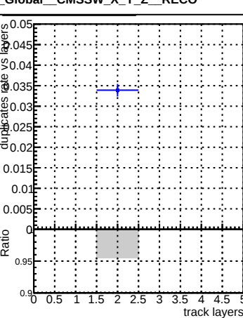
Duplicates Rate vs
