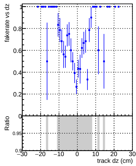
Fake rate vs dz Legend: DQM_V0001_R000000001_Global_CMSSW_X_Y_Z_RECO
