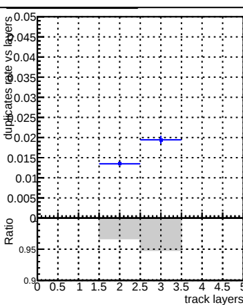
Duplicates Rate vs track layers
