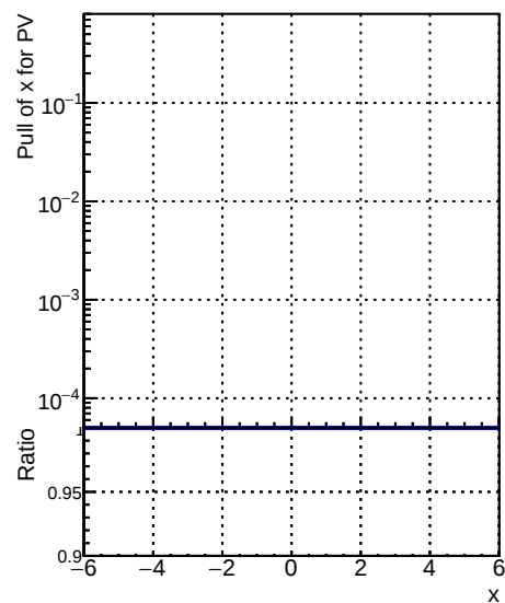
RecoPVAssoc2GenPVMatched_PullX
