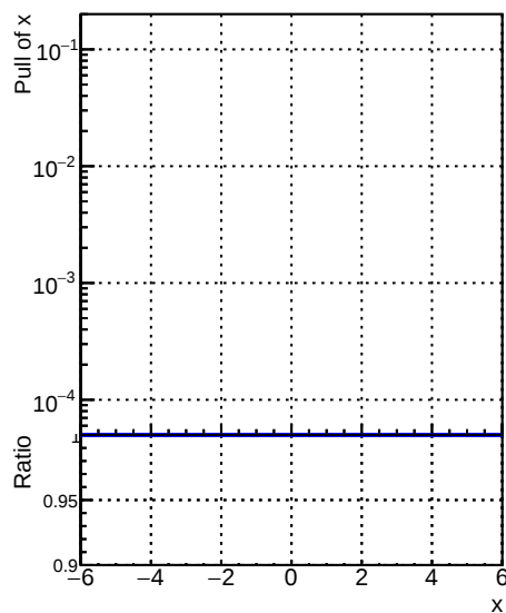
RecoAllAssoc2GenMatched_PullX
