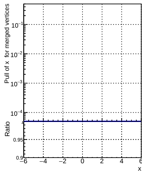
RecoAllAssoc2GenMatchedMerged_PullX
