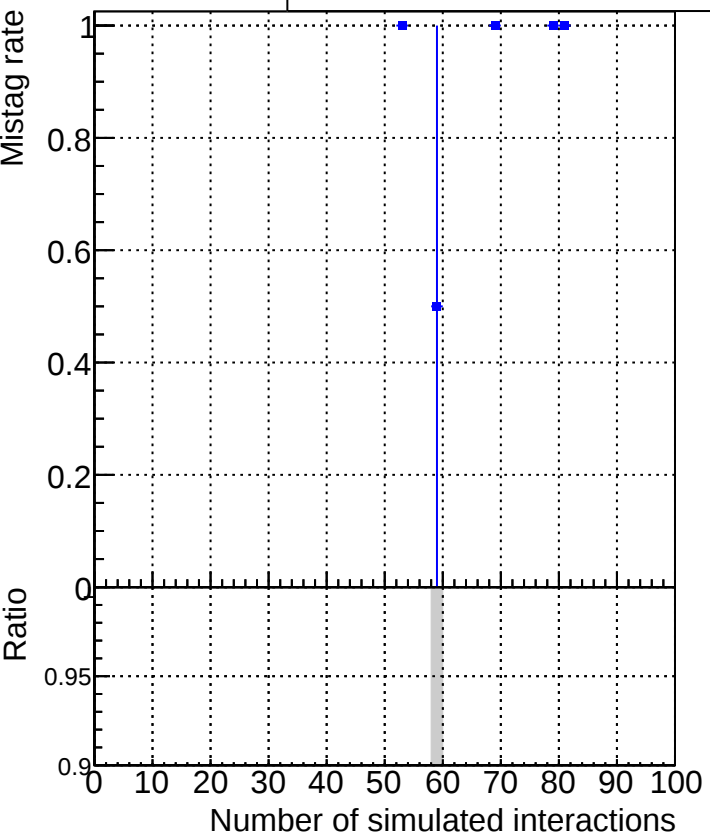
DQM_V0001_R000000001_Global_CMSSW_X_Y_Z_RECO
