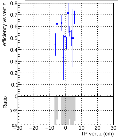
Efficiency vs. TP vert z ■ DQM_V0001_R0000000001_Global_CMSSW_X_Y_Z_RECO
