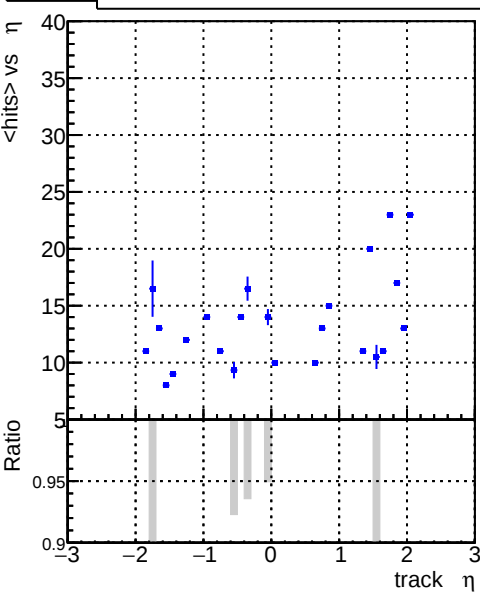
mean hits vs \eta DQM_V0001_R0000000001_Global_CMSSW_X_Y_Z_RECO
