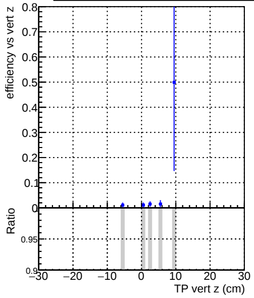
Efficiency vs TP vert z (cm) DQM_V0001_R0000000001_Global_CMSSW_X_Y_Z_RECO
