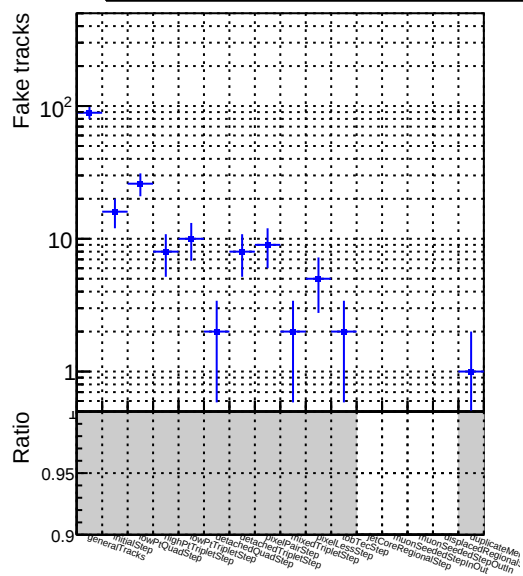
Number DQM_V0001_R000000001_Global_CMSSW_X_Y_Z_RECO
