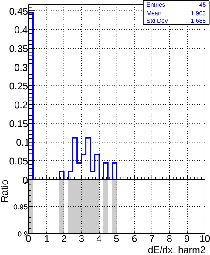
DQM_V0001_R000000001_Global_CMSSW_X_Y_Z_RECO
