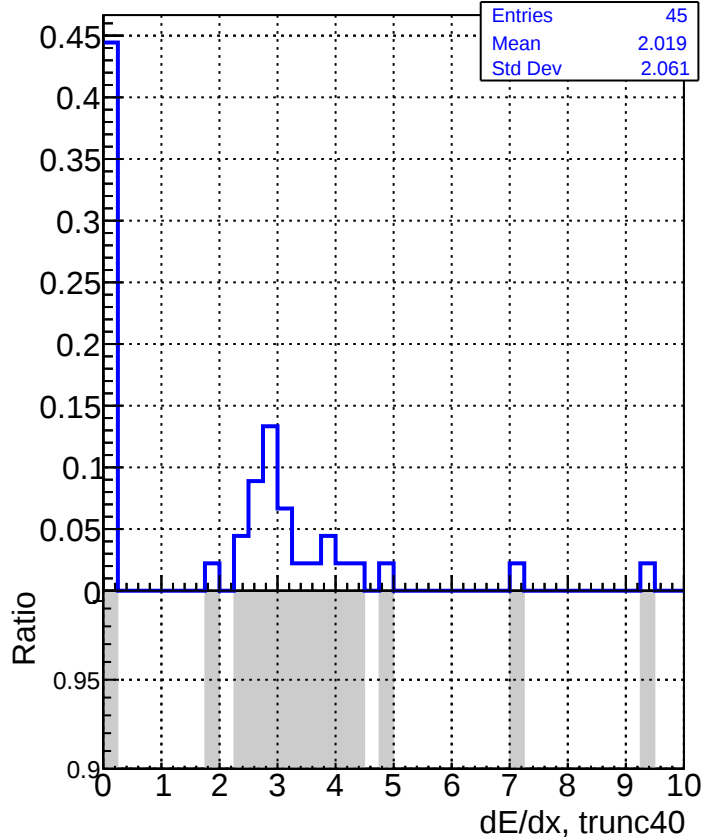
DQM_V0001_R000000001_Global_CMSSW_X_Y_Z_RECO
