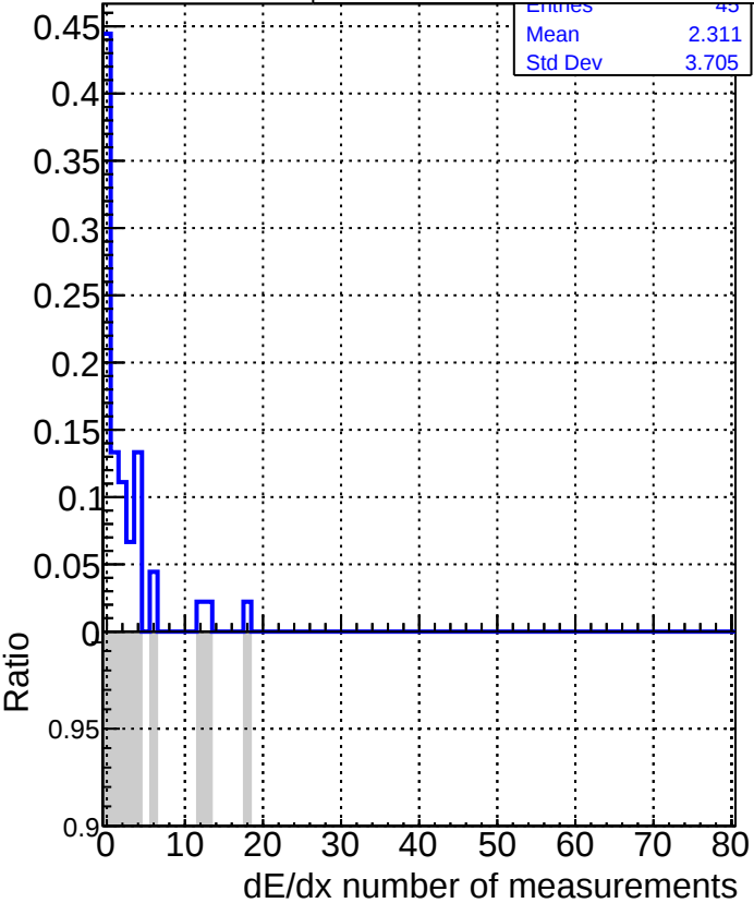
DQM_V0001_R000000001_Global_CMSSW_X_Y_Z_RECO
