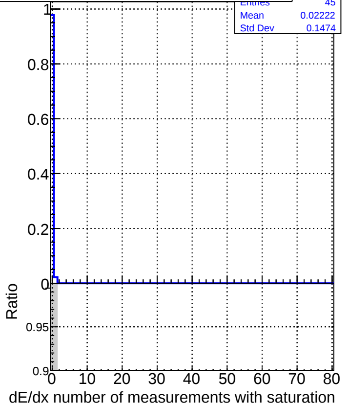
DQM_V0001_R000000001_Global_CMSSW_X_Y_Z_RECO
