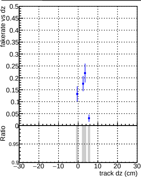
Fake rate vs dz Legend: DQM_V0001_R000000001_Global_CMSSW_X_Y_Z_RECO
