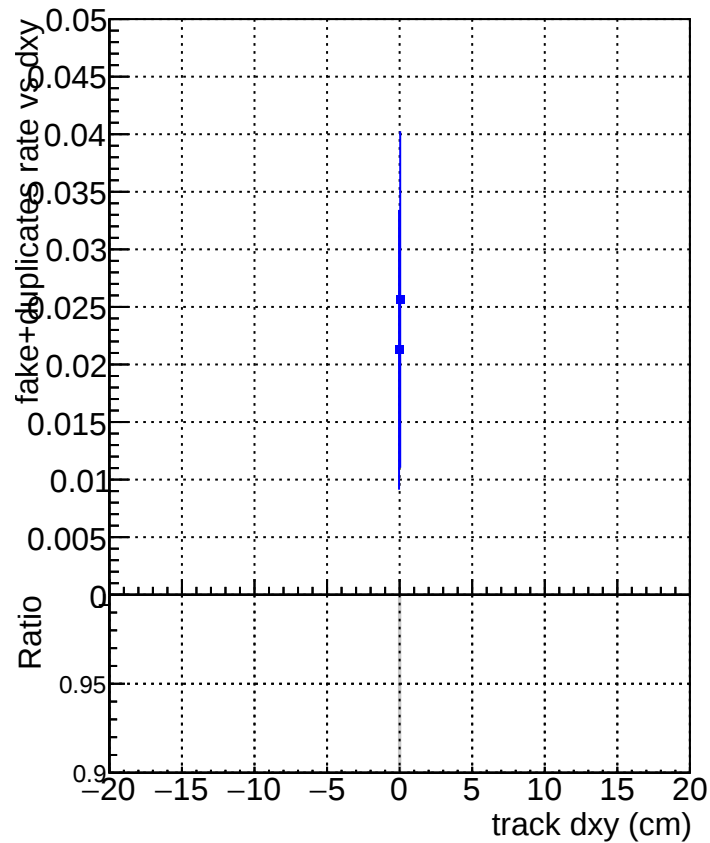
DQM_V0001_R000000001_Global_CMSSW_X_Y_Z_RECO
