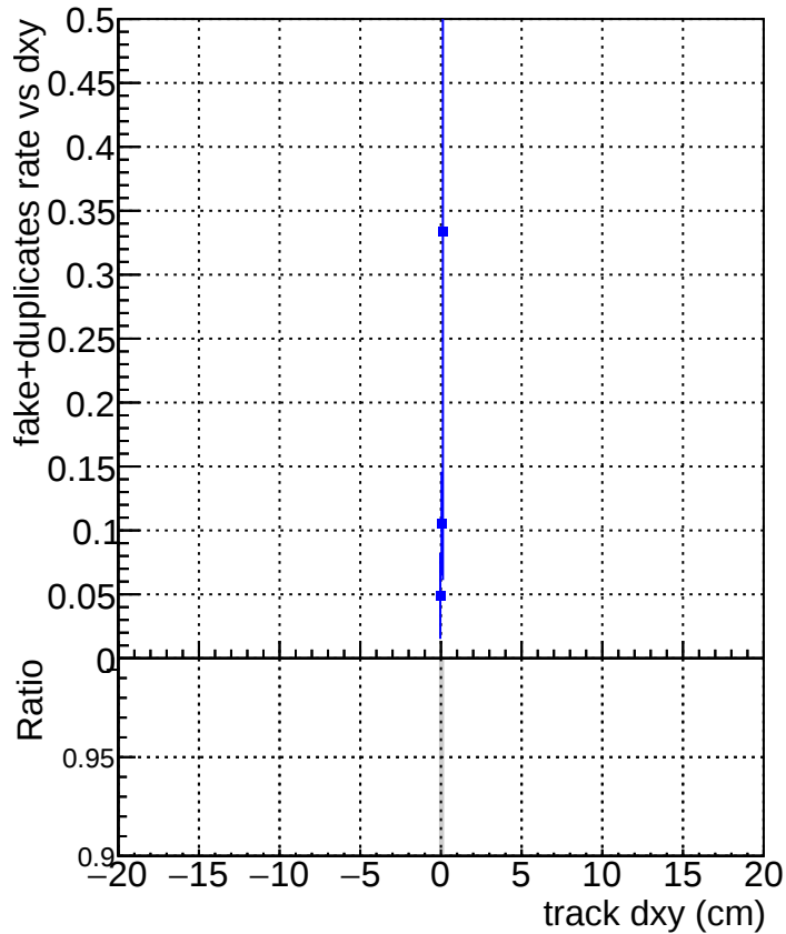
DQM_V0001_R000000001_Global_CMSSW_X_Y_Z_RECO
