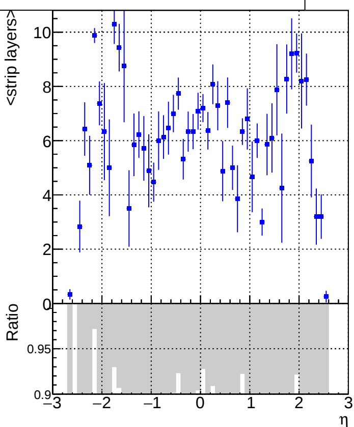
DQM_V0001_R000000001_Global_CMSSW_X_Y_Z_RECO
