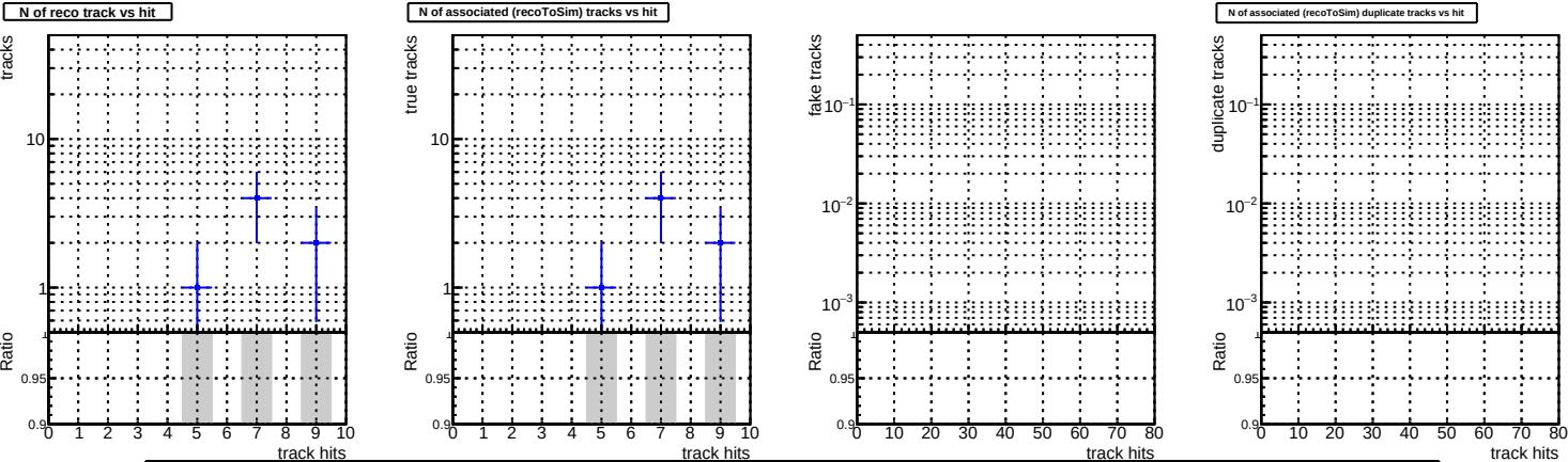
DQM_V0001_R000000001_Global_CMSSW_X_Y_Z_RECO
