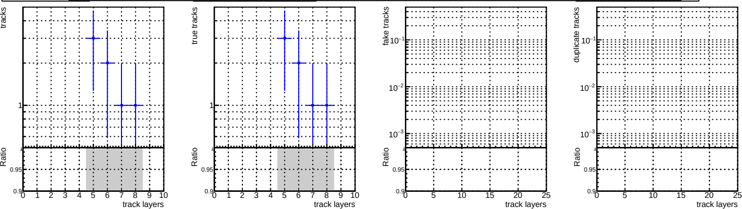
DQM_V0001_R000000001_Global_CMSSW_X_Y_Z_RECO
