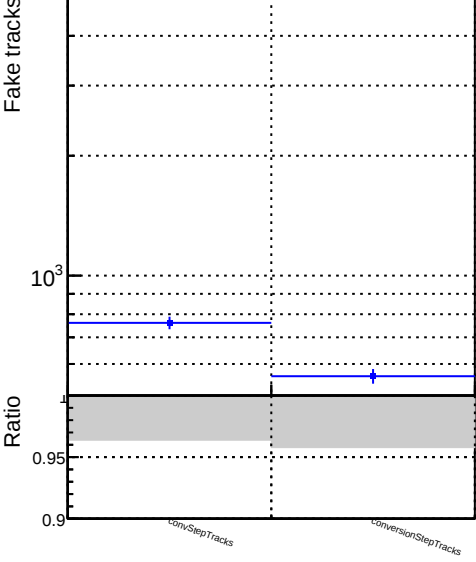
Number of tracks vs collection DQM_V0001_R000000001_Global_CMSSW_X_Y_Z_RECO
