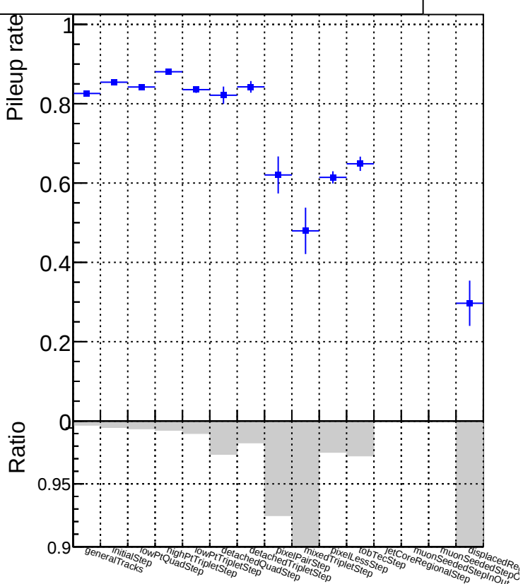
DQM_V0001_R000000001_Global_CMSSW_X_Y_Z_RECO
