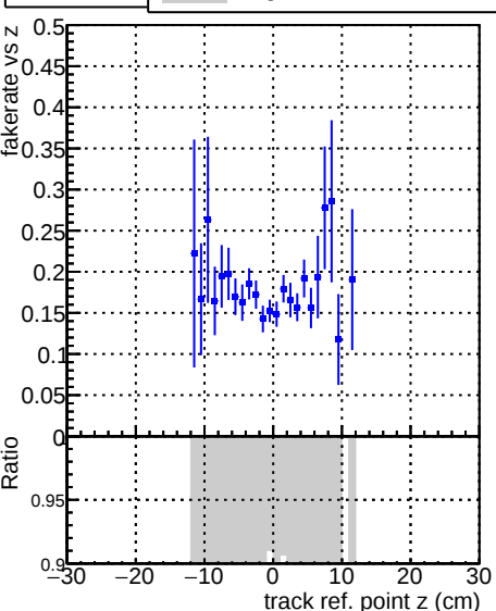
Fake rate vs DQM_V0001_R000000001_Global_CMSSW_X_Y_Z_RECO
