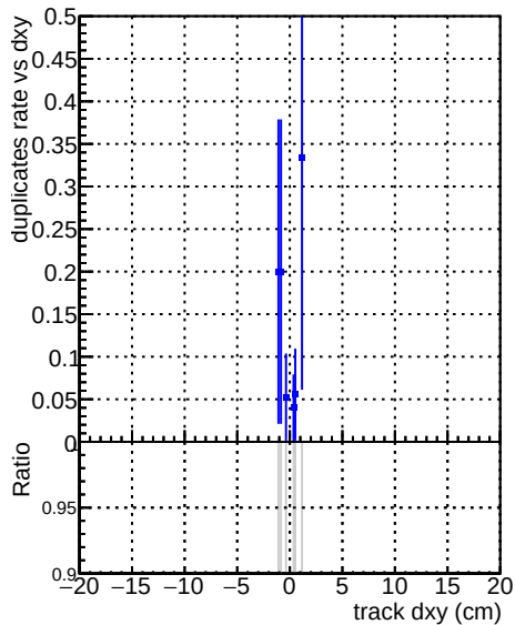
DQM_V0001_R000000001_Global_CMSSW_X_Y_Z_RECO
