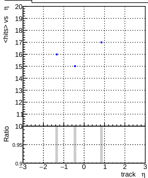
mean hits vs \eta DQM_V0001_R0000000001_Global_CMSSW_X_Y_Z_RECO
