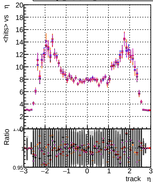
mean hits vs \eta DOM CKFEE1 1000evt DOM CKFEE2 1000evt DOM CKFEE3 1000evt DOM TESTOLHIT 1000evt DOM TESTOLHIT 1000evt-50000t
