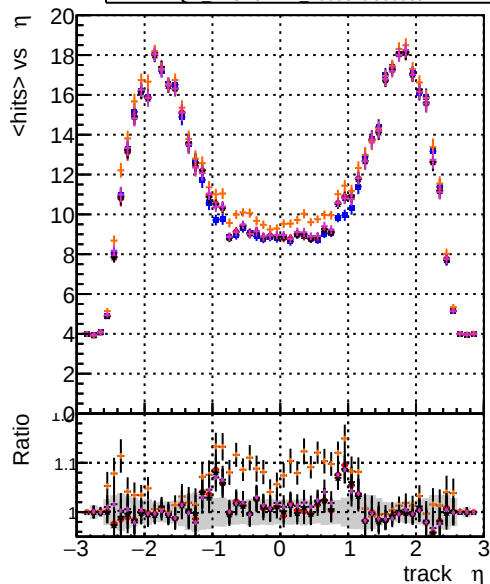
mean hits vs \eta DOM CKEFFit 1000evt DOM CKEFFit 10000evt DOM CKEFFit 100000t DOM TESTOLHIT 1000evt DOM TESTOLHIT 10000evt DOM TESTOLHIT 100000t
