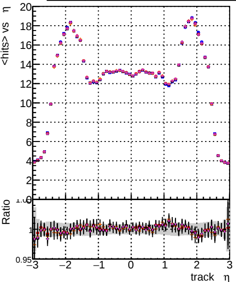
mean hits vs \eta DOM CKFit 1000evt DOM CKFit 10000evt DOM CKFit 100000t DOM TESTOLHIT 1000evt DOM TESTOLHIT 10000evt DOM TESTOLHIT 100000t
