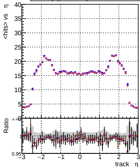
mean hit DOM CKFEEL 1000evt DOM CKFEEL 100000t DOM MCFEEL 100000t DOM TESTOLHIT 100000t DOM TESTOLHIT 100000t
