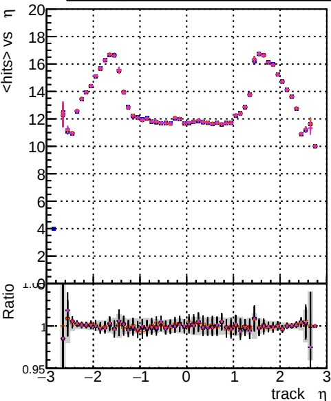
mean hits vs \eta DOM CKFEE1 1000evt DOM CKFEE2 1000evt DOM CKFEE3 1000evt DOM TESTOLHIT 1000evt DOM TESTOLHIT 1000evt-50000t
