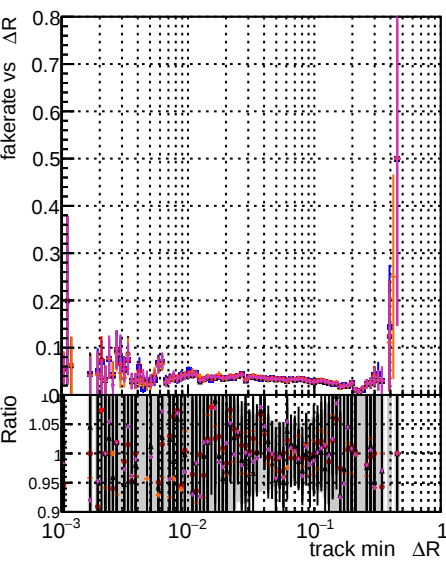
Fake rate vs \Delta R(\text{track, jet}) Legend: DOM CKFit 1000evt DOM CKFit 10000evt DOM CKFit 100000evt DOM TESTOLHIT 10000evt DOM TESTOLHIT 50000evt
