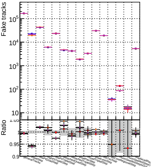
Number Line Style Label Black line with triangle DOM MKFITREFIT 1000evt Orange line with cross DOM TESTOLHIT 1000evt Purple line with cross DOM TESTOLHIT 1000evt-50000t
