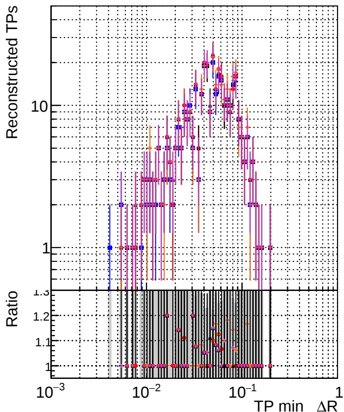
N of associated tracks (simToReco) vs dR
