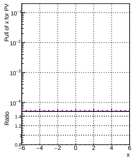
Legend: RecoPVAssoc: RecoAllAssoc: RecoAllAssocMerged: Data: Fit: 1000evt: 10000evt: 100000evt: 500000t
