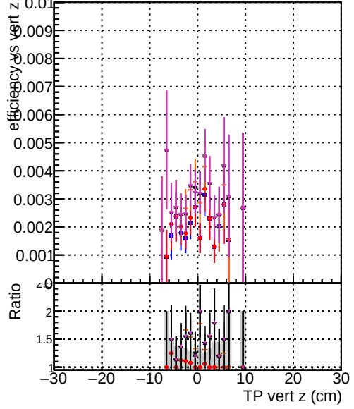
Efficiency vs vertpos — DOM CKFEEL 1000evt — DOM CKFEEL 1000evt — DOM CKFEEL 1000evt — DOM TESTOLHIT 1000evt — DOM TESTOLHIT 1000evt-50000t
