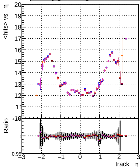
mean hits vs \eta DOM CKFit 1000evt DOM CKFit 10000evt DOM CKFit 100000evt DOM TESTOLHIT 1000evt DOM TESTOLHIT 1000000t
