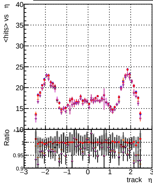
mean hit \eta DOM CKFit 1000evt DOM CKFit 100000t DOM MCFit 1000evt DOM TESTOLHIT 1000evt DOM TESTOLHIT 1000evt-50000t
