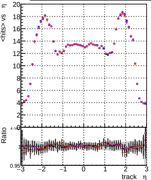
mean hits vs \eta DOM CKFEREL 1000evt DOM CKFEREL 1000evt DOM CKFEREL 1000evt DOM TESTOLHIT 1000evt DOM TESTOLHIT 1000evt-50000t
