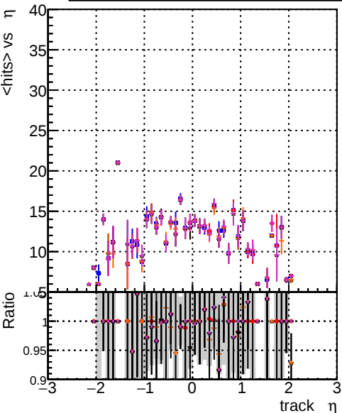
mean hits vs \eta DOM CKFEREEL 1000evt DOM CKFEREEL 1000evt DOM CKFEREEL 1000evt DOM TESTOLHIT 1000evt DOM TESTOLHIT 1000evt-50000t
