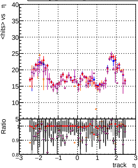
mean hit DOM CKFEEL 1000evt DOM CKFEEL 100000t DOM MCFEEL 100000t DOM TESTOLHIT 100000t DOM TESTOLHIT 100000t-50000t
