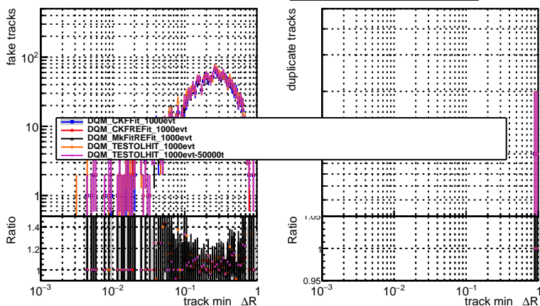
N of associated (recoToSim) loopers tracks vs dR
